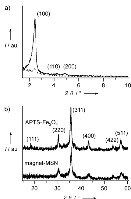
Figure 3. a) Low-angle X-ray diffraction (XRD) patterns of linker-MSN (—) and magnet-MSN (----) powders. b) High-angle XRD patterns of APTS-coated Fe 3 O 4 nanoparticles (top) and magnet-MSN (below).
