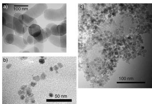
Figure 2. TEM images of a) linker-MSNs, b) APTS-coated Fe 3 O 4 nanoparticles, and c) Fe 3 O 4 -capped magnet-MSNs.
